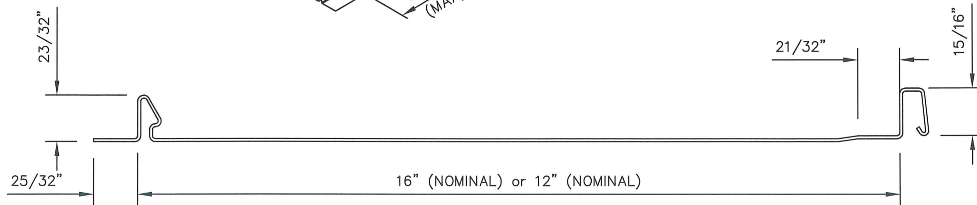
PANEL PROFILE
